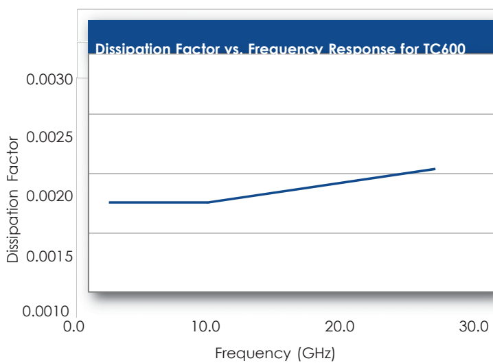
Figure 2 Demonstrates the stability of dissipation factor across frequency. This characteristic demonstrates the inherent robustness of Rogers' laminates across frequency, providing a stable platform for high frequency applications where signal integrity is critical to the overall performance of the application. Resonant Cavity Methods yielded slightly lower dissipation factor results than IPC 650-TM 2.5.5.5. Df across 1.8 GHz to 25.6 GHz averaged 0.0017 in the Z-Axis. Dielectric loss best correlates with Z-Axis (E-field perpendicular to the board) as the signal propagation down the length of the board maintains the E-Field perpendicular to the plane of the board (right hand rule), such as a microstrip or stripline design.
