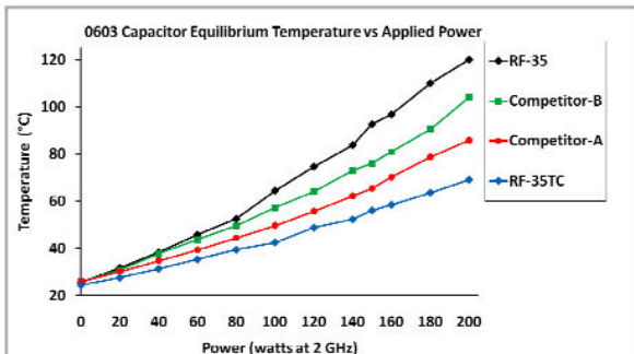
Maximum temperature as a function of applied power for a microstrip and 0603 capacitor assembled on RF-35TC, RF-35 and two competitive materials.
